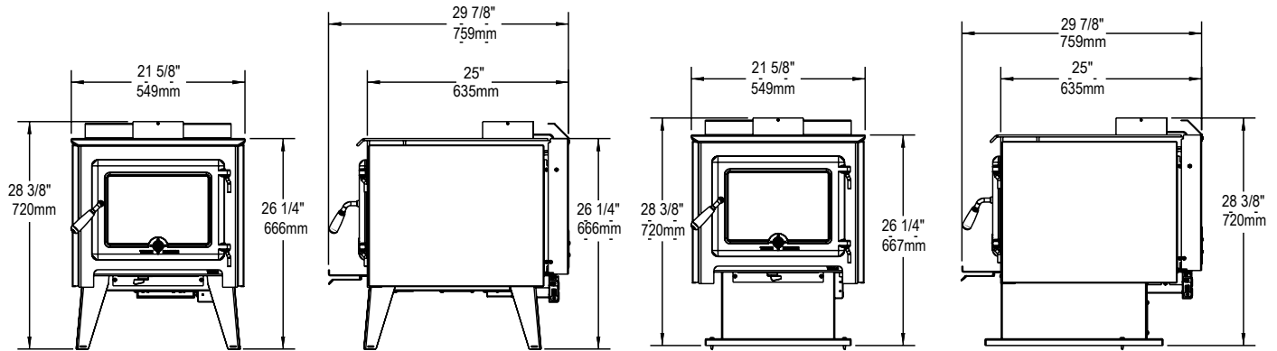
Figure 1: TN25C Dimensions.
